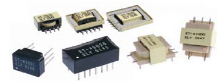
TELECOM TRANSFORMERS
