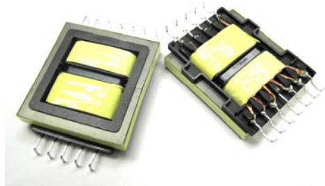
LLC RESONANT POWER TRANSFORMERS FOR TV THIN TRANSFORMERS
